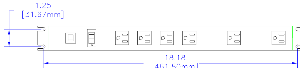
TOP VIEW
